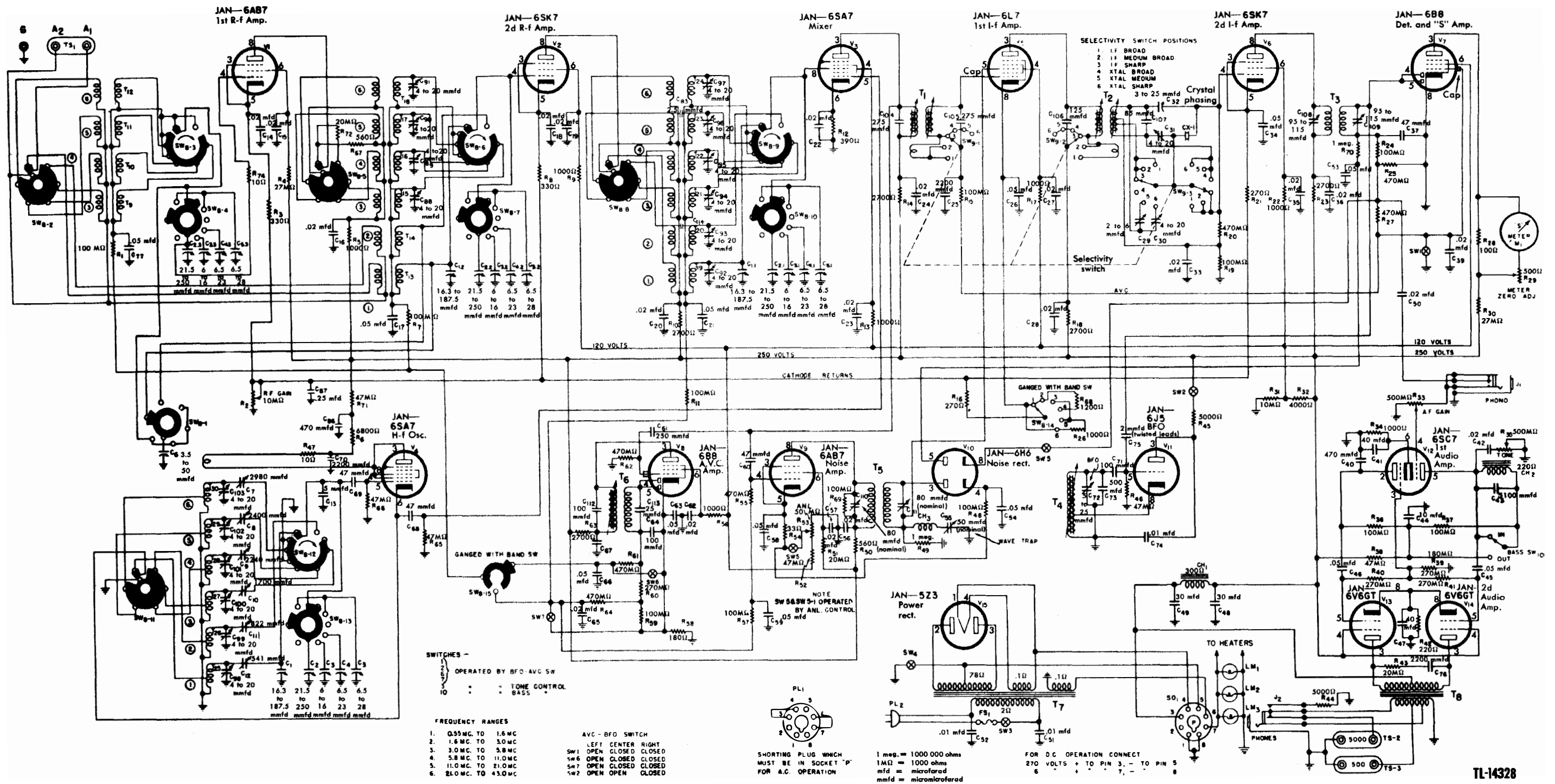
Figure 27. Radio Receiver AN/GRR-2, schematic diagram.
