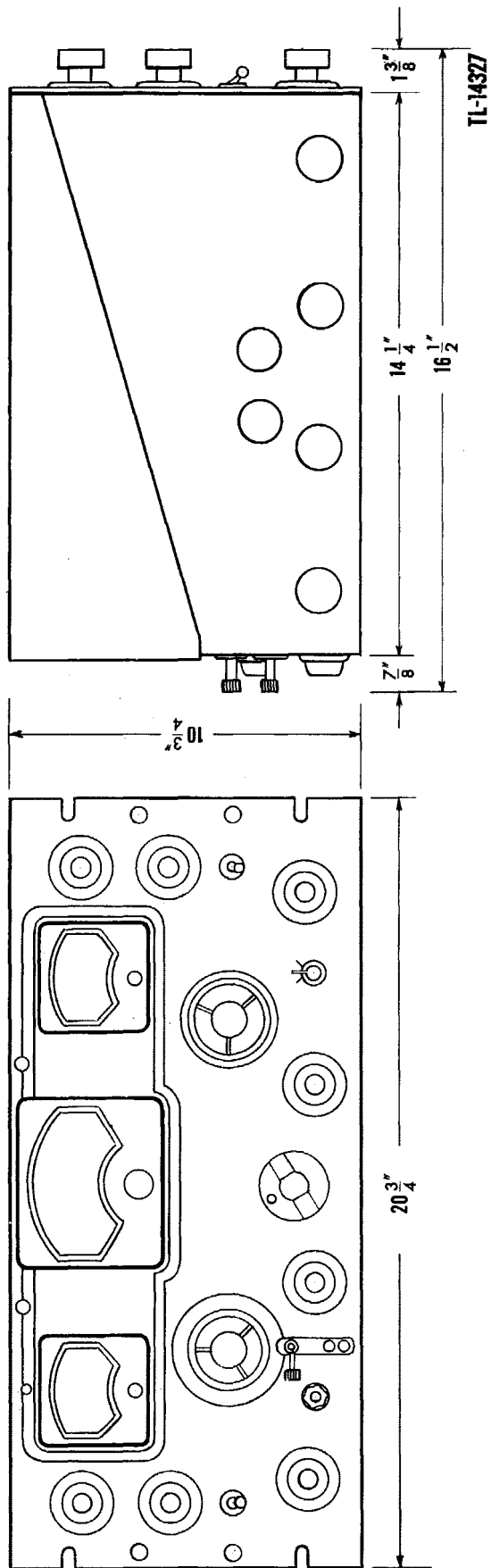
Figure 26. Dimensional drawing.
