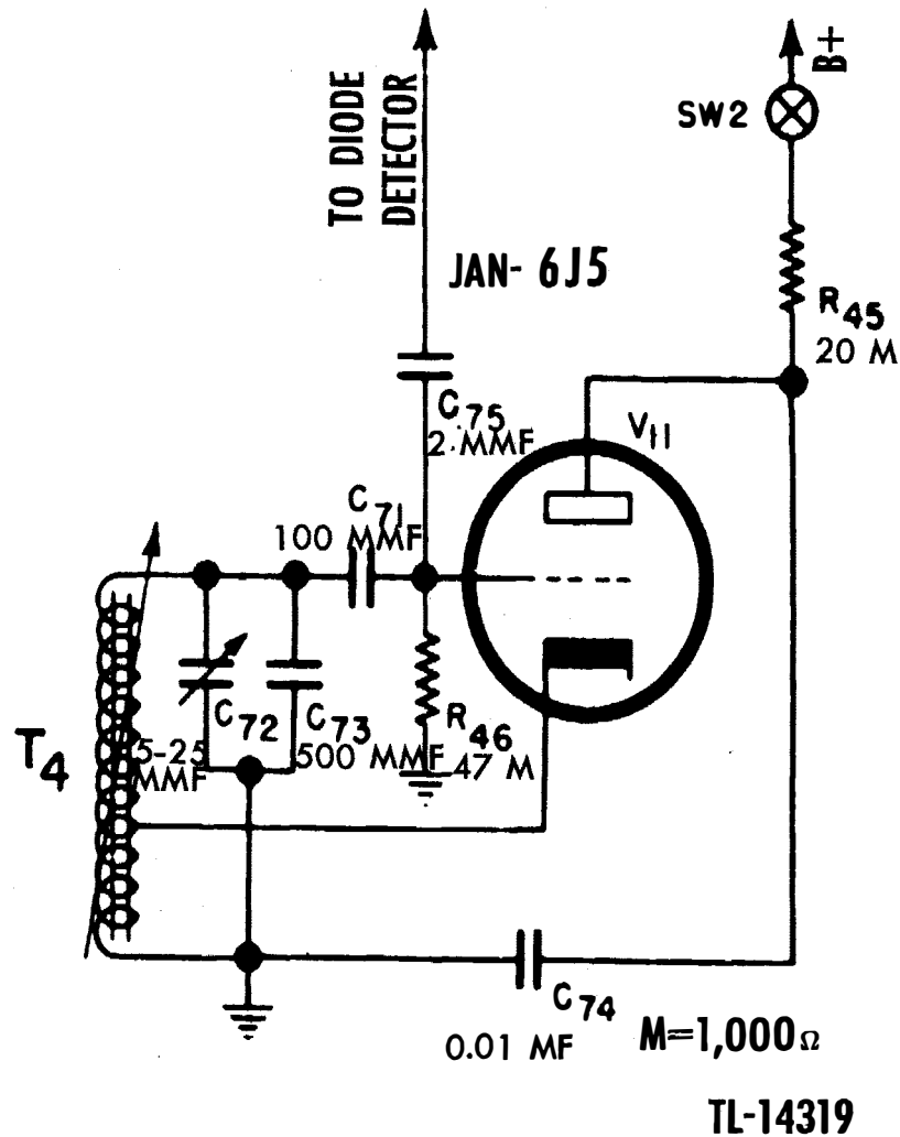
Figure 19. Beat-frequency oscillator, schematic.
