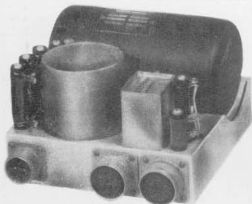
Dynamotor DY-30/APN-19
