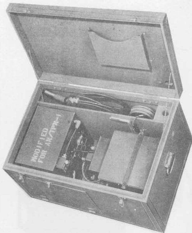
AN/TPN-1 packed in Case CY-21/TPN-1 is air transportable and easily assembled.
